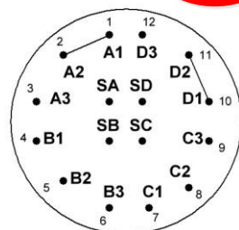
SW3: Tone
